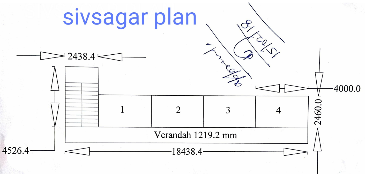
Proposed Ground Floor & 1st Floor Plan (Area=72.91 sq.m/each floor)
